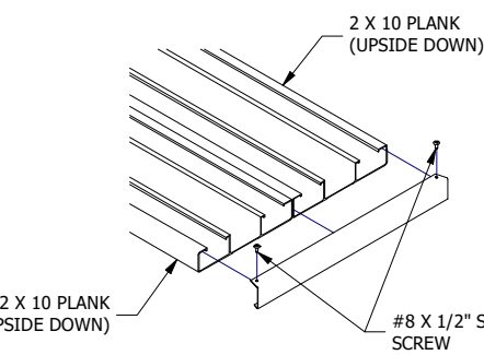
TYPICAL 2 X 10 PLANK ATTACHMENT
