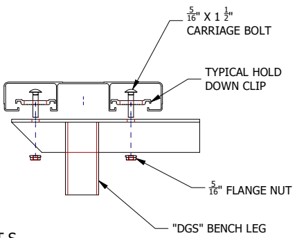
TYPICAL 2 X 10 PLANK ATTACHMENT
