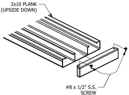
TYP. DBL. 2 X 10 END CAP ATTACHMENT
